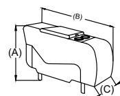
A. TOTAL HEIGHT BACK - 25"(63.5cm) B. TOTAL DEPTH - 38.25"(97cm) C. TOTAL WIDTH - 12.5"(31.75cm)
