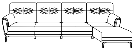
3 STR + RH / LH DAYBED TW - 110" (279.5cm) / ISW - 94" (239cm) DBTW - 32" (81.5cm) / DBISW - 24" (61cm) DBTD - 70" (178cm) / DBSD - 54" (137cm)
