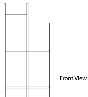
Wall Hung Racking Unit - Large W - 660/440mm, H - 1325mm, D - 330mm
