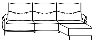
3 STR + RH/LH DAYBED TW - 102"(259cm)/ISW - 90"(228.5cm) DBTW - 36.5"(93cm)/DBISW - 30"(76cm) DBTD - 67.25"(171cm)/DBSD - 49.5"(126cm)
