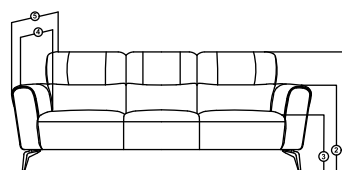
1. TOTAL HEIGHT - 37.5"(95.5cm) 2. ARM REST HEIGHT - 25.75"(65.5cm) 3. SEAT HEIGHT - 17.5"(44.5cm) 4. SEAT DEPTH - 22"(56cm) 5. TOTAL DEPTH - 39"(99cm) 6. LEG HEIGHT - 6.25"(15.8cm)
