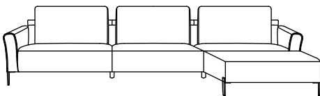
3 STR + RH/LH DAYBED TW - 122" (310cm) / ISW - 109" (277cm) DBTW - 42.5" (108cm) / DBISW - 36" (94.5cm) DBTD - 70.5" (179cm) / DBSD - 54" (137cm)
