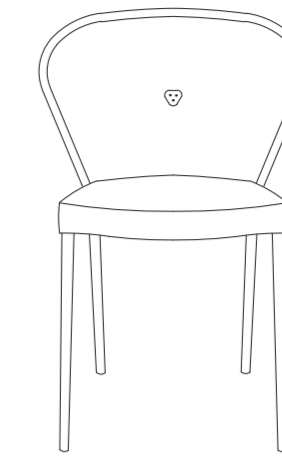
CROWN Total Height - 32" Total Depth - 20" Total Width - 17" Seat Height - 17.5" Seat Depth - 17.5" Inside Seat Width - 17"
