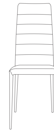
CARLTON Total Height - 41" Total Depth - 23" Total Width - 17.5" Seat Height - 19" Seat Depth - 16.5" Inside Seat Width - 17.5"
