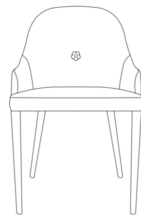
HYATT Total Height - 33" Total Depth - 22" Total Width - 20.5" Arm rest Height - 21.5" Seat Height - 18.5" Seat Depth - 17.5" Inside Seat Width - 17"
