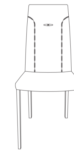
RITZ Total Height - 41.5" Total Depth - 20.5" Total Width - 18" Seat Height - 19" Seat Depth - 16.5" Inside Seat Width - 18"
